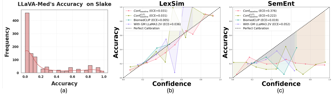
Figure 8: (a) Histogram on the frequency of LLaVA-Med’s accuracy on Slake. Reliability diagrams for UQ of LLaVA-Med on Slake by (b) LexSim, and (c) SemEnt. Each diagram shows plots and the respective ECE for the confidence reported by the baseline Conf_{baseline} , its calibrated version Conf_{baseline}^{(1/T)} , and the proposed approach (2) for calibration with different grounding models.
