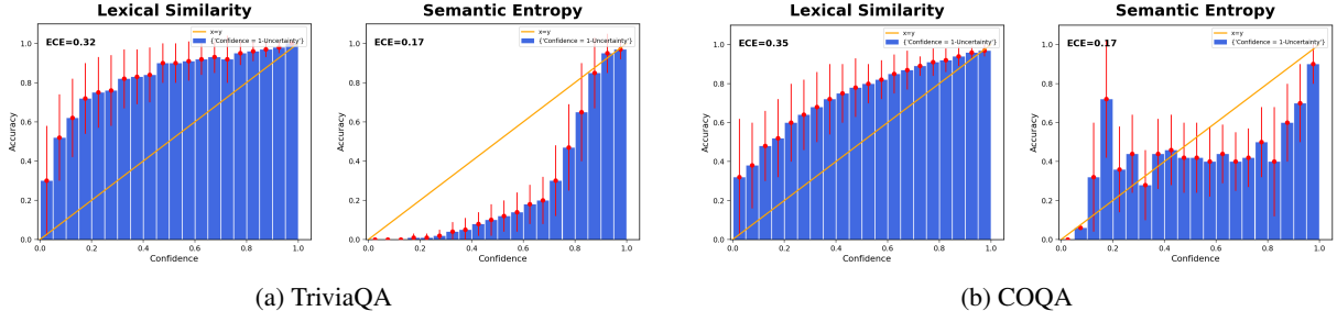
Figure 4: Reliability diagrams with the expected accuracy of LLaMA-2-13B on TriviaQA and COQA plotted as a function of the model’s confidence predicted by two SOTA self-consistency-based UQ approaches. A perfect calibration between the model’s accuracy and the predicted confidence would result in red points, representing the average accuracy for each confidence bin, lying on the x = y axis with low variance.
