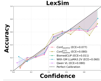
Figure 12: Reliability diagram and ECE comparison of LexSim with different GM in the proposed calibration approach for Gemini on the medical dataset Slake.
