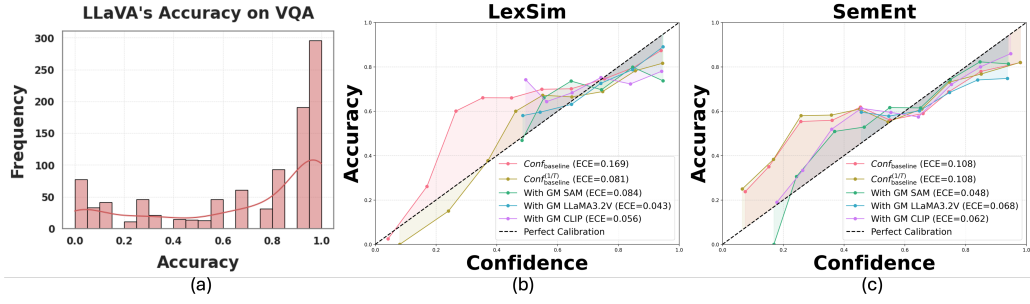
Figure 3: (a) Histogram on the frequency of LLaVA’s accuracy on VQA. Reliability Diagrams for UQ of LLaVA on VQA by (b) LexSim, and (c) SemEnt baseline. Each diagram shows plots and the respective ECE for the confidence reported by the baseline Conf_{baseline} , its calibrated version Conf_{baseline}^{(1/T)} , and the proposed approach 2 for calibration with different GM.
