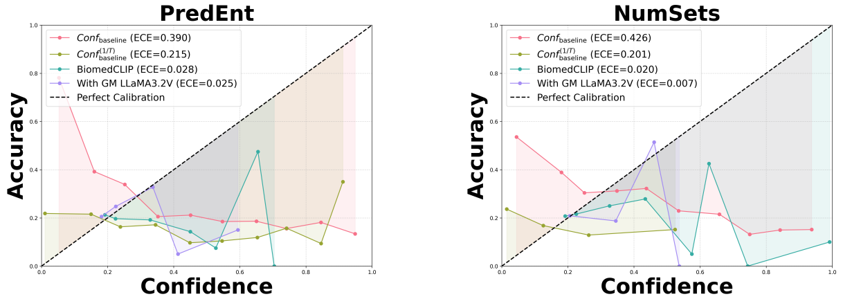
Figure 9: Reliability diagrams for UQ by PredEnt and NumSets baselines for LLaVA on the VQA dataset. Each diagram shows plots and ECE for the confidence reported by the baseline Conf_{baseline} , its calibrated version Conf_{baseline}^{(1/T)} , and the proposed approach (2) for calibration with different grounding models.
