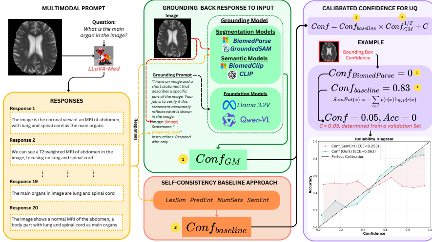
Figure 2: Conf_{baseline} : confidence from a self-consistency UQ baseline such as LexSim (Fomicheva et al., 2020), PredEnt (Malinin and Gales), NumSets (Kuhn et al., 2023), SemEnt (Kuhn et al., 2023), etc. on a VLM such as LLaVA-Med. Conf_{GM}^{1/T} : temperature-scaled calibrated confidence of grounding model on the accuracy of the generated responses. A grounding model can be as simple as the CLIP-based model, that provides its confidence in terms of a similarity score between embeddings of the generated response and the input image (e.g. BiomedCLIP), a detection model for response on the input image reporting its confidence on the detected bounding box (e.g. BiomedParse), or a foundation model that provides its verdict – a confidence score in [0, 1] – on the relevance of the generated response to the input image (e.g. LLaMA 3.2V, Qwen VL, etc.). Conf (2) is the proposed calibrated confidence score for UQ of VLMs resulting in substantially lower ECE than the baseline.
