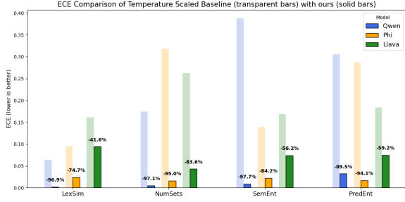
Figure 11: Temperature-scaled baselines’ comparisons of ECE ( \downarrow ) with Clip as the GM in the proposed approach for different VLMs – Qwen, Phi, Llava – on GQA.
